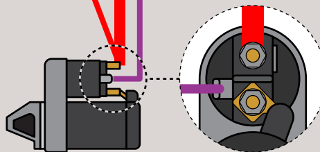
EME # STARTER MOTOR
